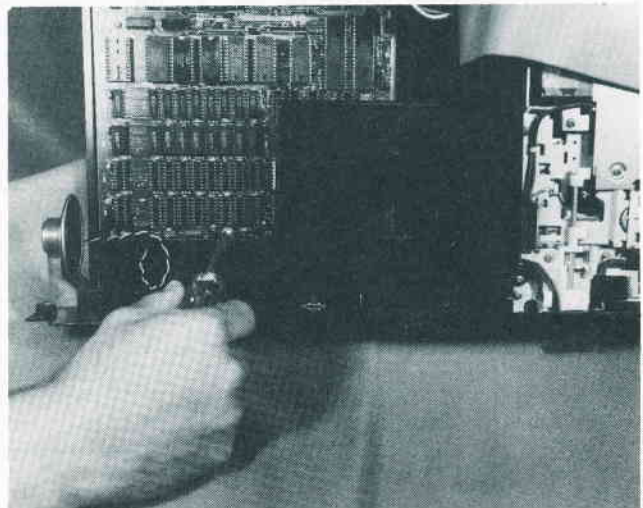
Fig. A-4. Remove the system-board mounting screws.
