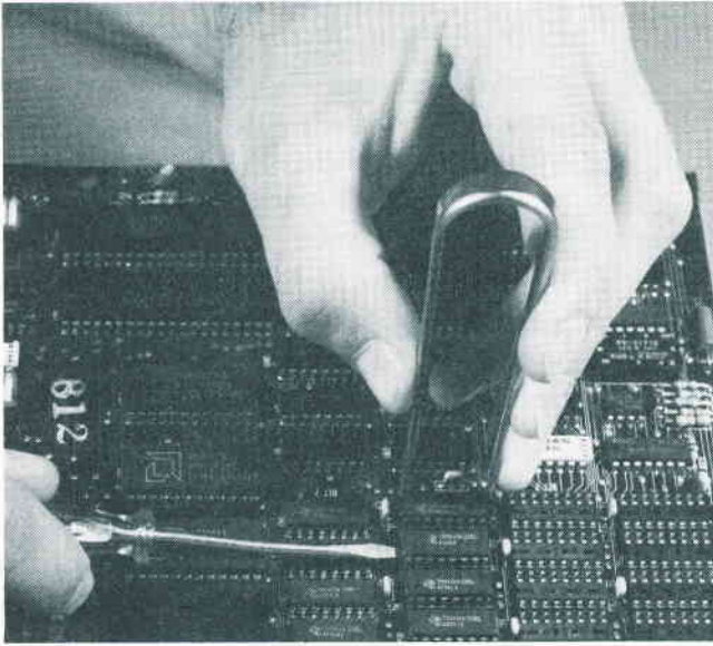
Fig. 3-8. ICs can be removed with a chip extractor or by gently prying up with a tiny screwdriver (tweaker).
