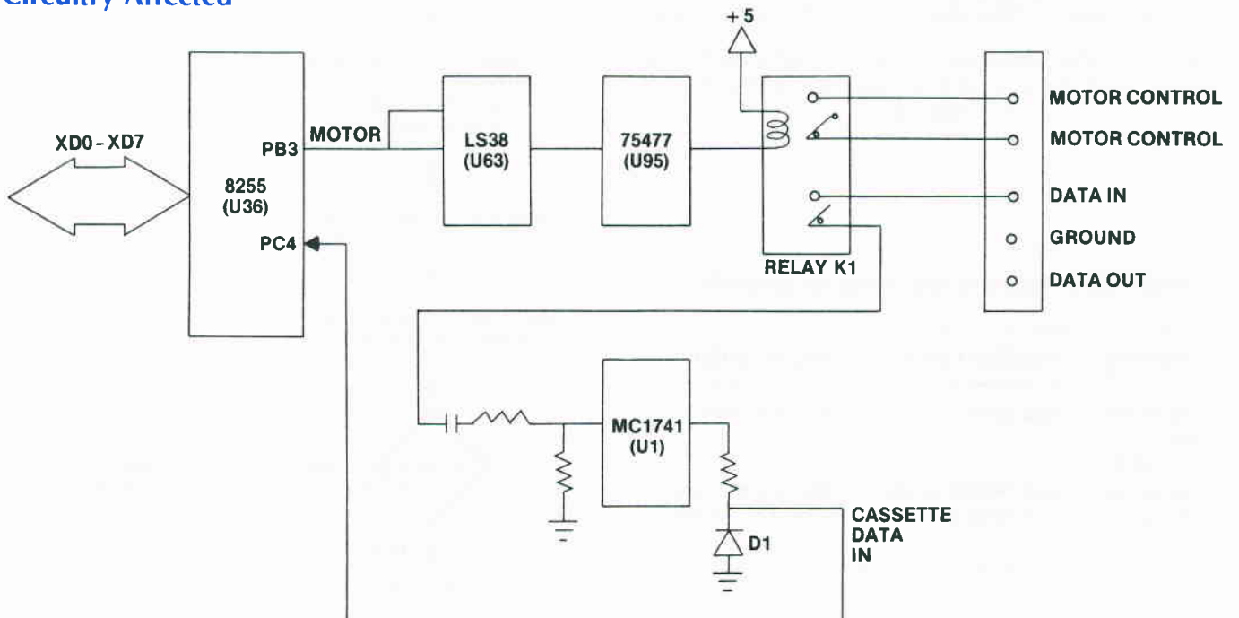
Fig. 4-44. Cassette data input circuitry.
