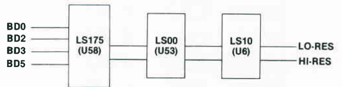
Fig. 4-25. Low-resolution graphics circuitry.
