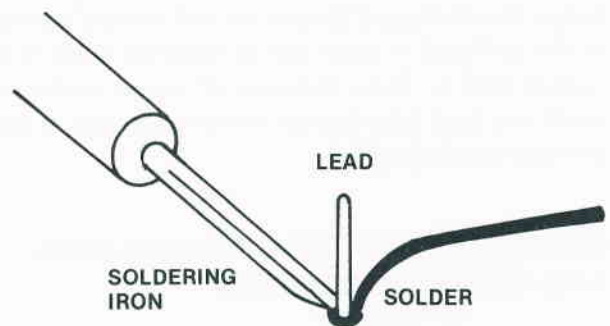
Fig. 6-28. Place the soldering iron on the opposite side of the lead from the solder.
