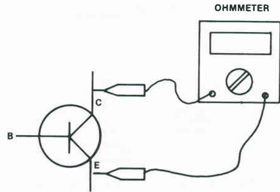
Fig. 6-22. A transistor can be tested using an ohmmeter placed across the collector-to-emitter junction.
