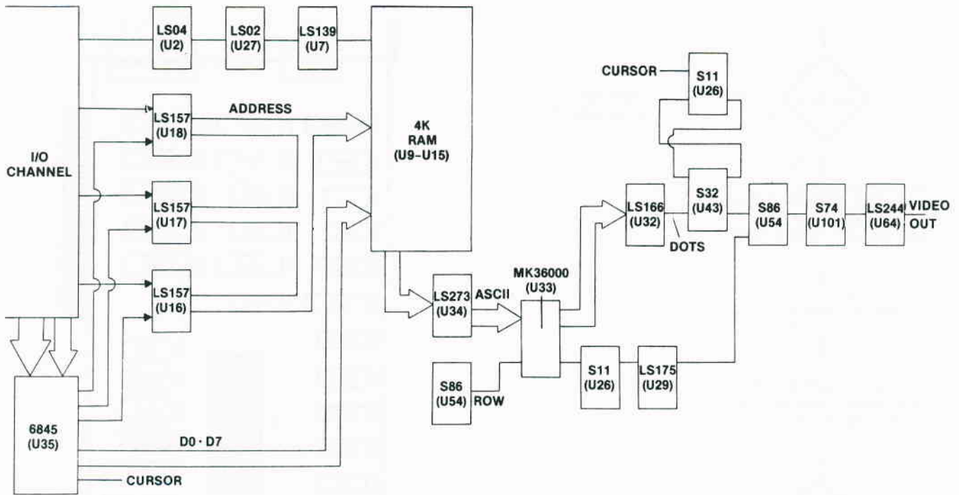
Fig. 4-19. Monochrome video circuitry.
