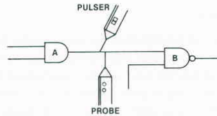
Fig. 6-9. Place the probe and the pulser on the AND gate output.
