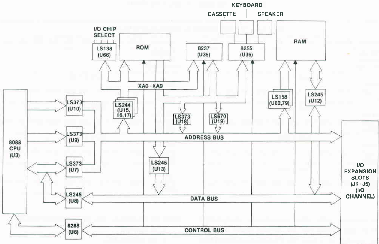
Fig. 2-17. The complete IBM PC bus structure.
