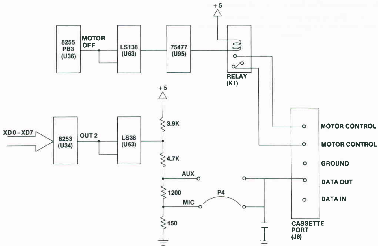
Fig. 4-46. Cassette data output circuitry.
