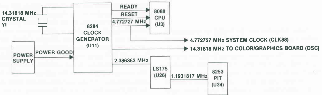
Fig. 2-9. The IBM PC clock circuitry.
