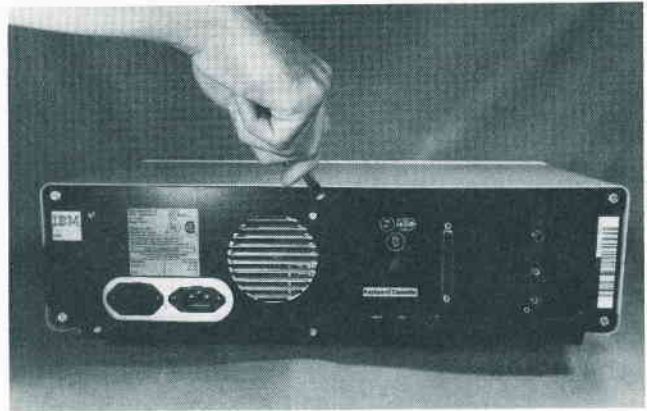
Fig. A-2. Remove these screws to disassemble the IBM PC.
