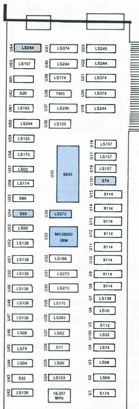
Fig. 4-18. Chip location guide. This represents the IBM PC monochrome adapter card and is a guide to help you find the chips of interest.
